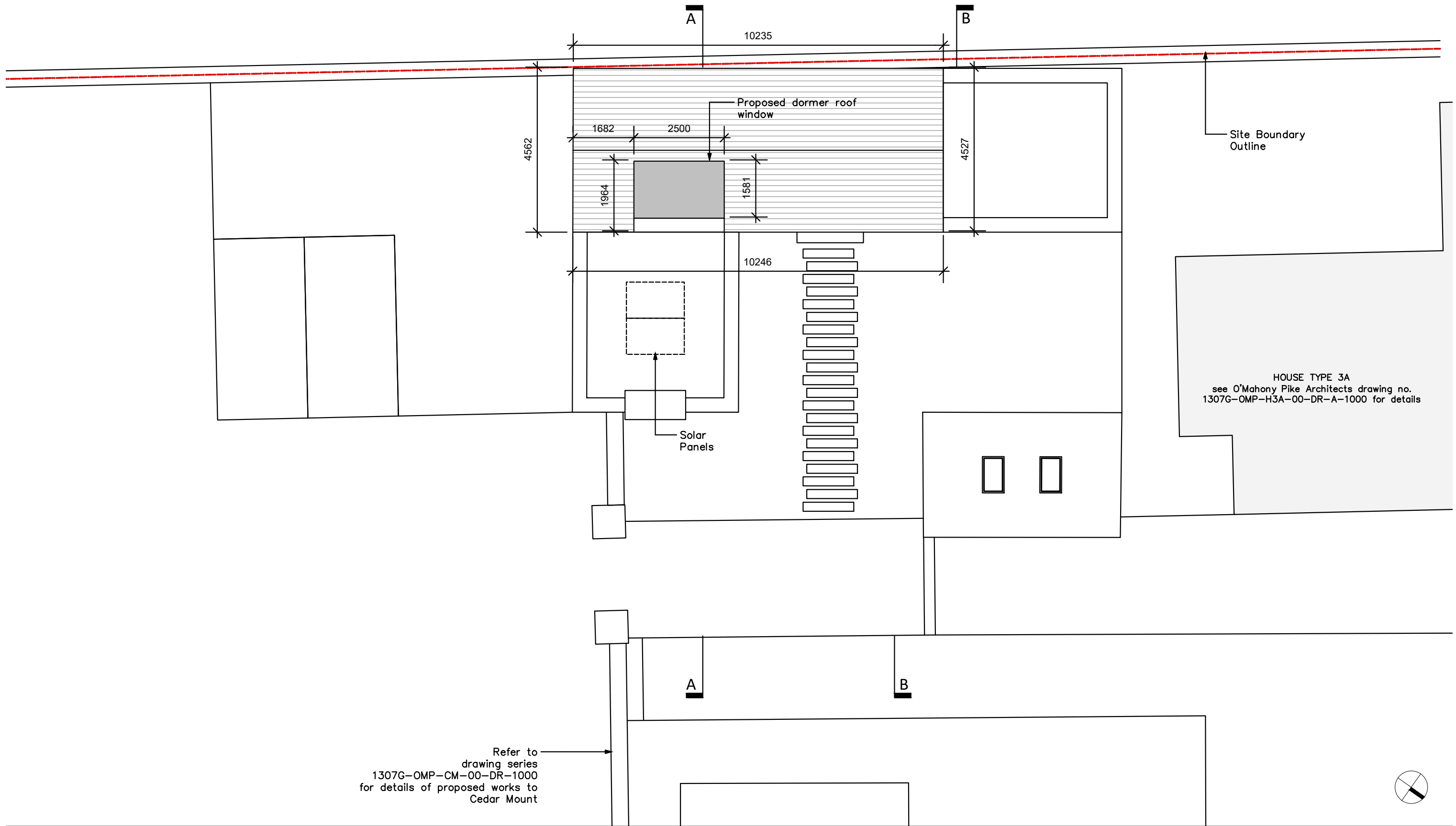
Coach House, Proposed Roof Plan
